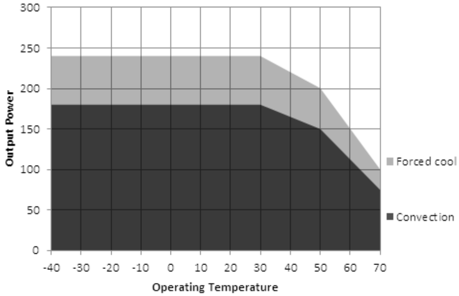
De-rating Curve- 12V for plain cover
