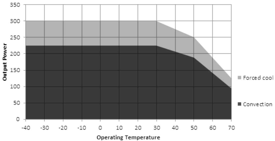
De-rating Curve- 15V for plain cover
