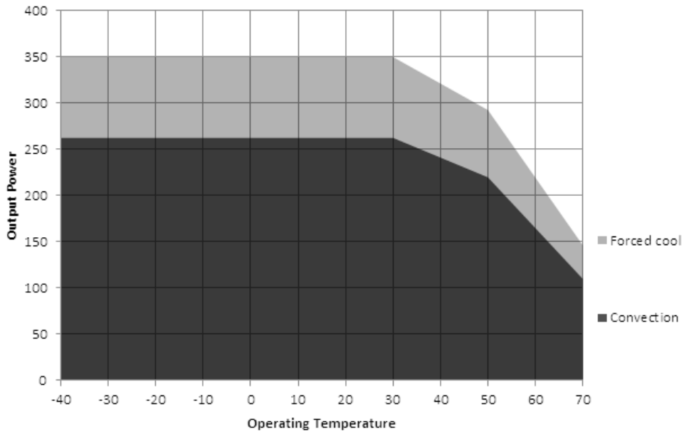
De-rating Curve- 15V for slotted cover
