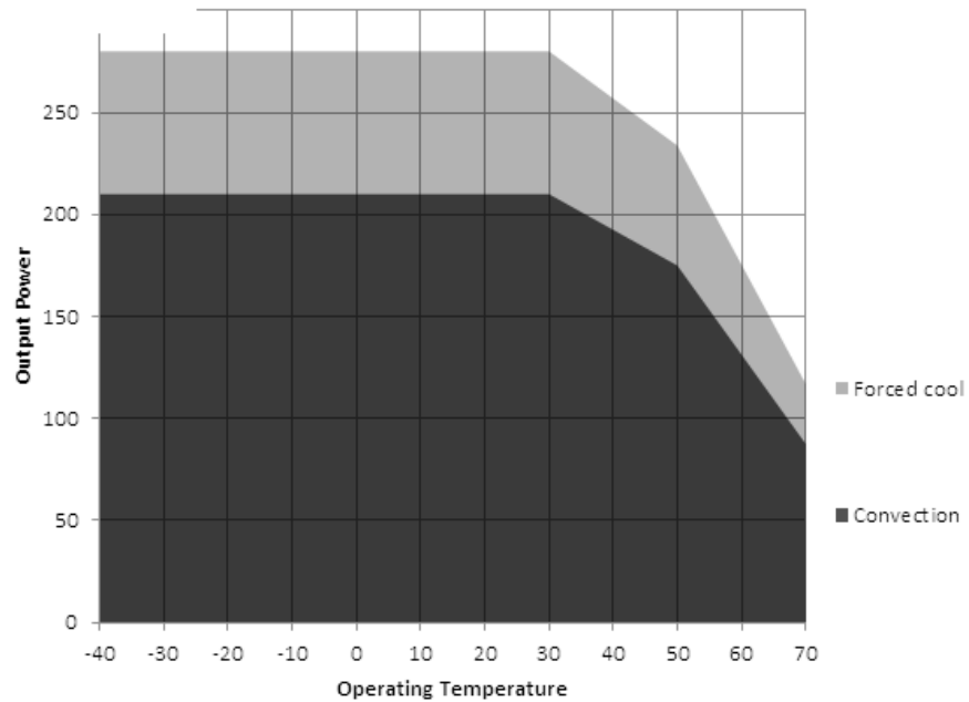
De-rating Curve- 12V for slotted cover
