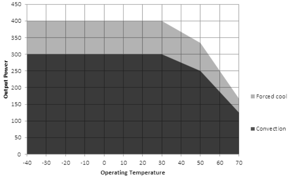
De-rating Curve 12V
