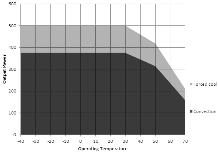
De-rating Curve 15V
