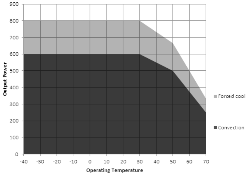
De-rating Curve- 24V & above
