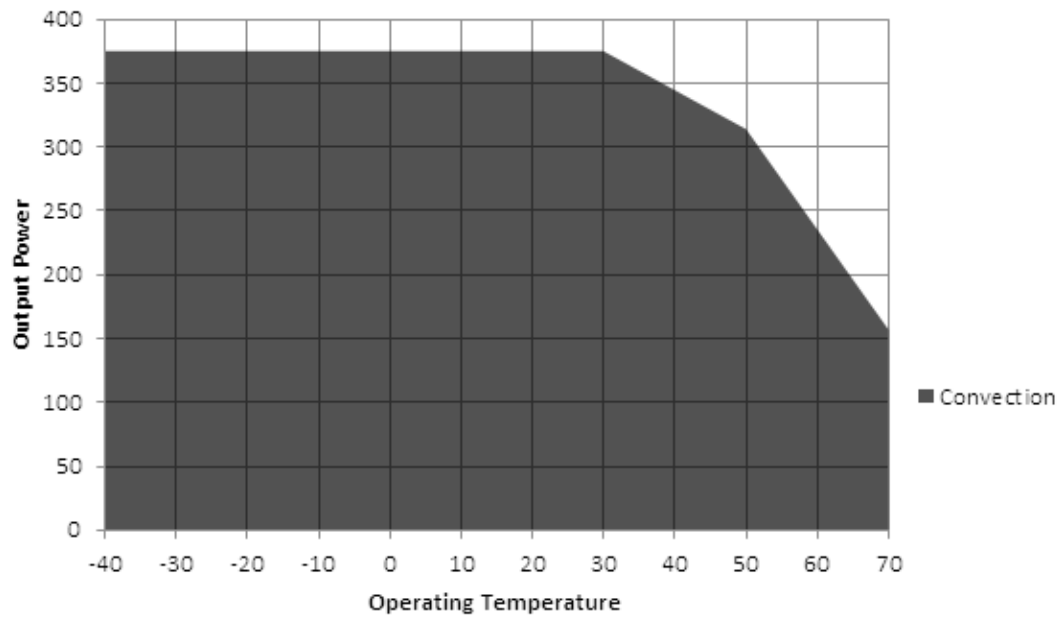
De-rating Curve 15V
