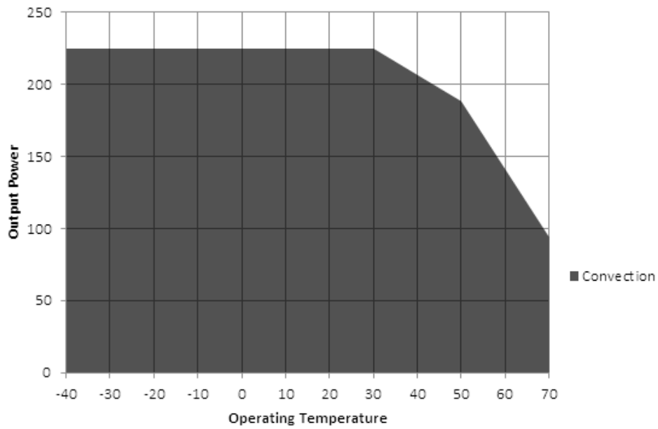
De-rating Curve- 15V for plain cover
