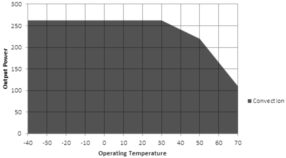
De-rating Curve- 15V for slotted cover
