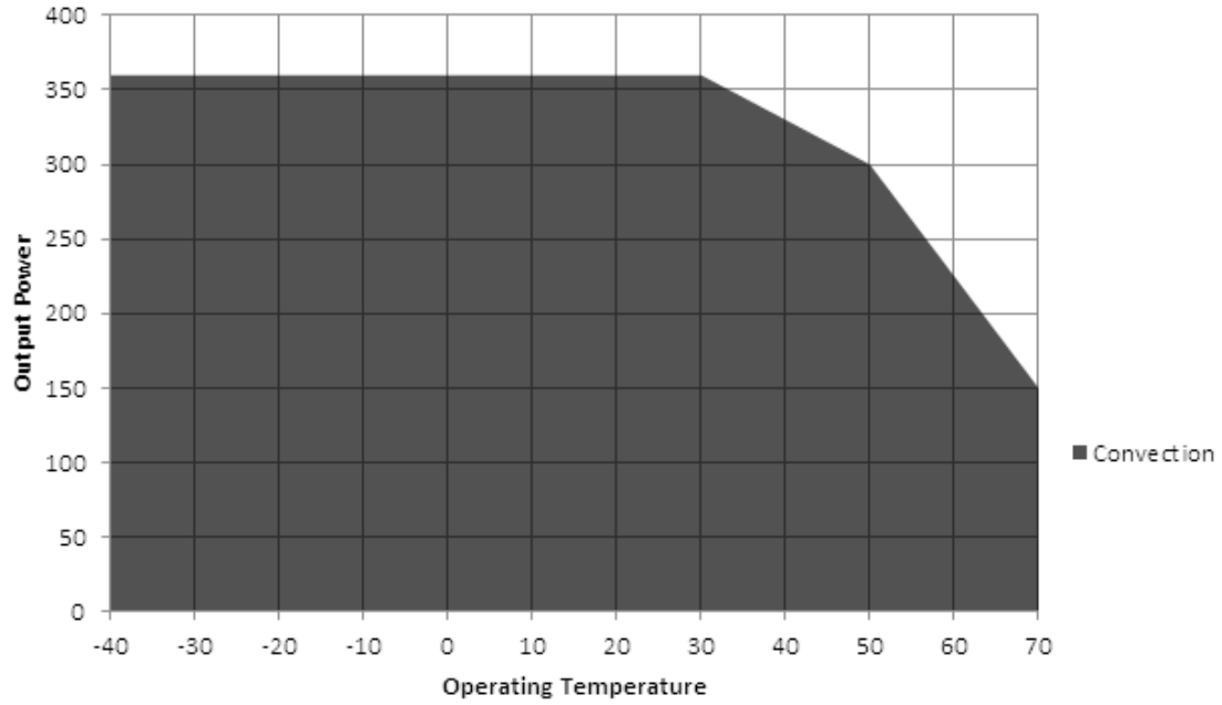
De-rating Curve- 24V & above for plain cover
