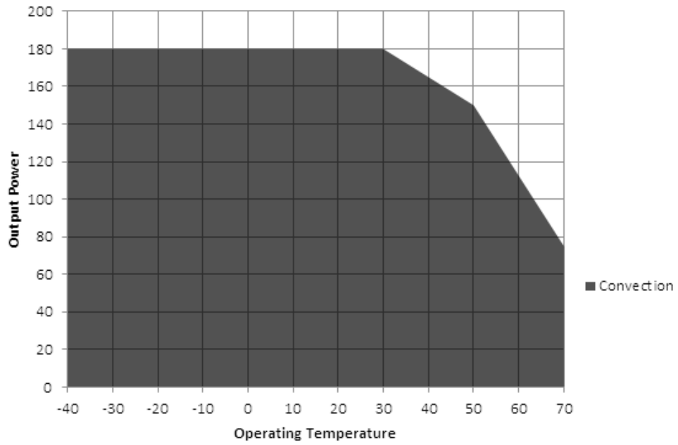
De-rating Curve- 12V for plain cover
