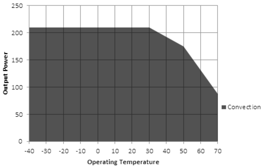
De-rating Curve- 12V for slotted cover
