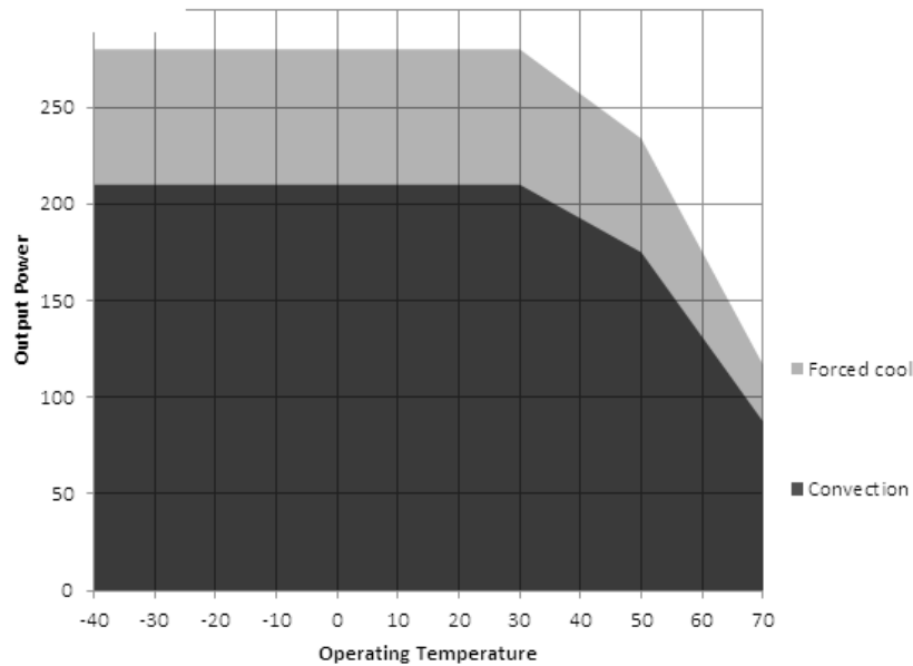
De-rating Curve- 12V for slotted cover
